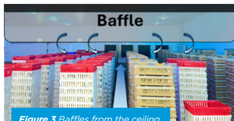
Figure 3 Baffles from the ceiling.
