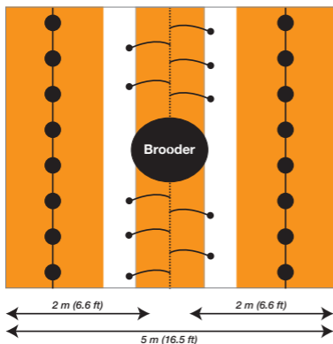
Typical spot brooding layout (per 1000 chicks).
